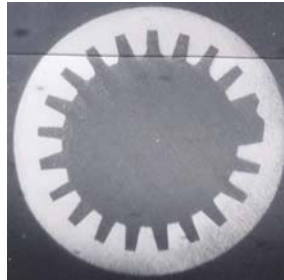
.025" x .050" Groove 19 Grooves
