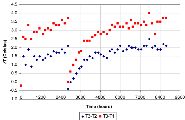
Figure 13. Low Temperature (Non-Condensable Gas) Measurements for Grade 5 Titanium Cylinder/CP-Titanium Screen/Water Heat Pipe 2, Operating at 550 K. Purged after 2837 hours of operation.
