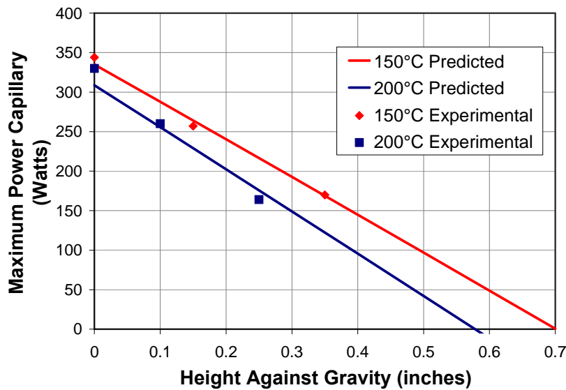
Figure 5. Typical Test Data and extrapolated performance (10°C Delta T). 23 Grooves, 0.51 mm x 1.02 mm (0.020" x 0.040"), Titanium/Water Heat Pipe.
