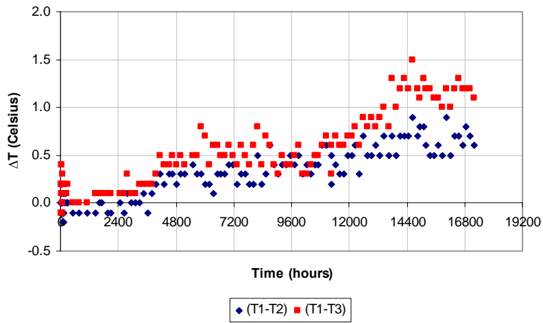
Figure 10. Low Temperature (Non-Condensable Gas) Measurements for Monel /Water Heat Pipe 106, Operating at 550 K.
