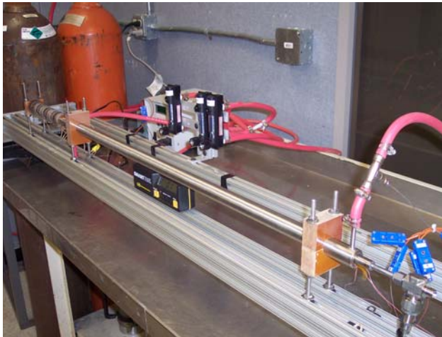
Figure 3. Heat Pipe Test Apparatus uses a gas gap calorimeter to remove heat.
