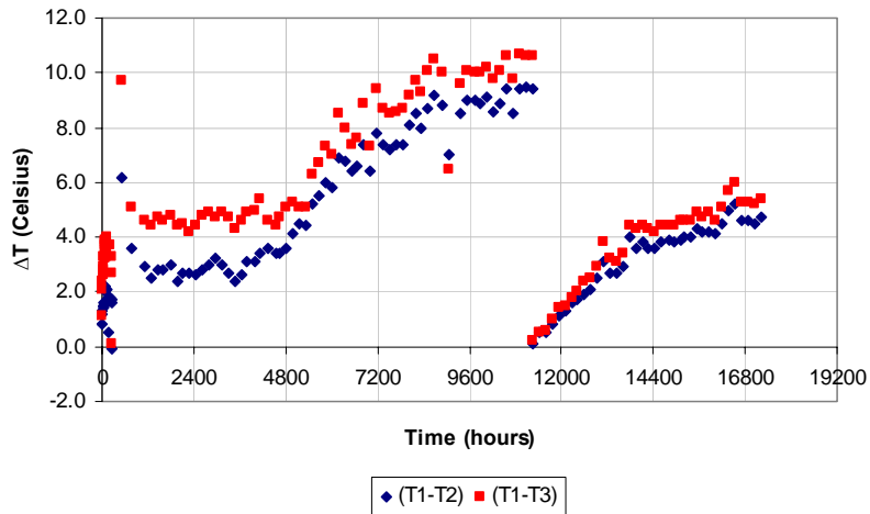
Figure 11. Low Temperature (Non-Condensable Gas) Measurements for CP Ti/Water Heat Pipe 103, Operating at 550 K. Second purge after 11,256 hours of operation.
