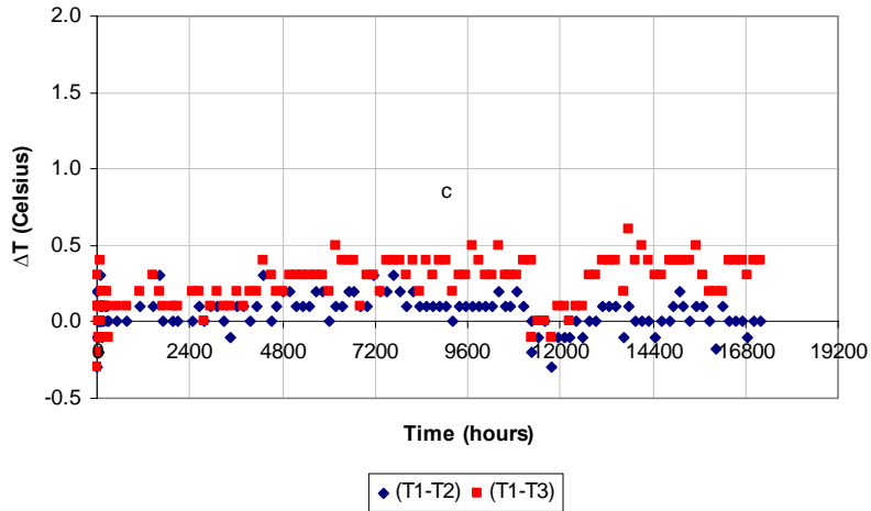
Figure 9. Low Temperature (Non-Condensable Gas) Measurements for Monel /Water Heat Pipe 105, Operating at 500 K.
