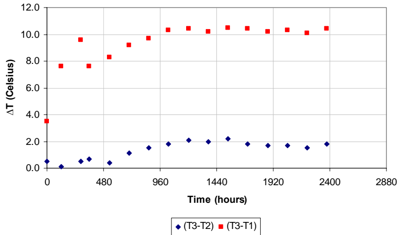
Figure 15. Low Temperature (Non-Condensable Gas) Measurements for Monel K-500 Envelope/Monel 400 Sintered Wick/Water Heat Pipe 20, Operating at 550 K.
