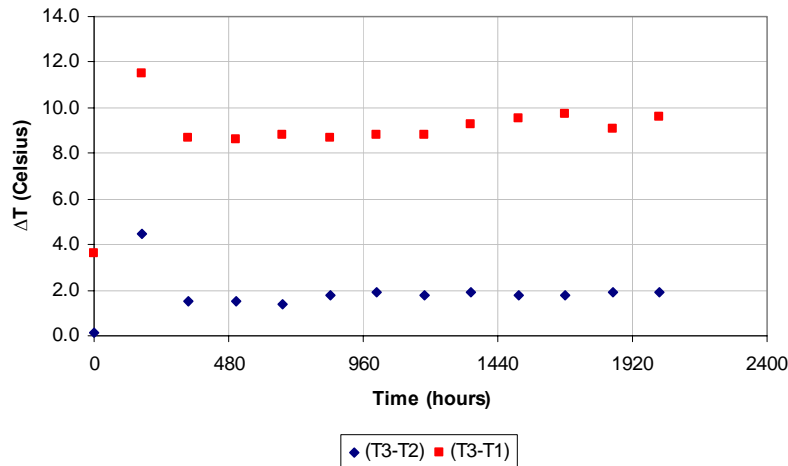
Figure 16. Low Temperature (Non-Condensable Gas) Measurements for Monel 400 Envelope/Monel 400 Sintered Wick/Water Heat Pipe 21, Operating at 550 K.
