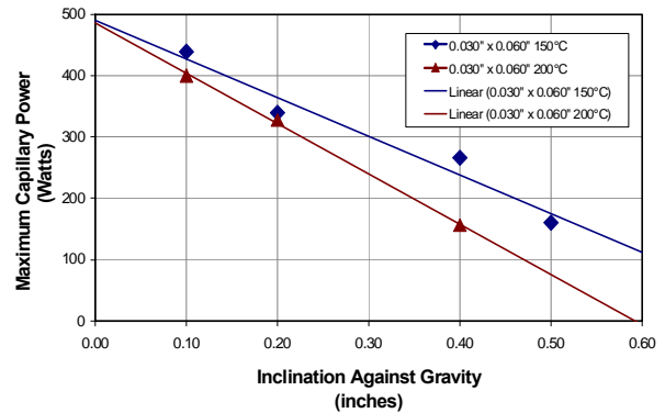
Figure 7. Typical Test Data and linear extrapolation (50 °C Delta T). 17 Grooves, 0.76 mm x 1.52 mm (0.030" x 0.060"), Titanium/Water Heat Pipe.
