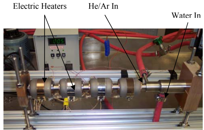
Figure 4. The evaporator has 4 electric heaters, with thermocouples welded in the gaps.
