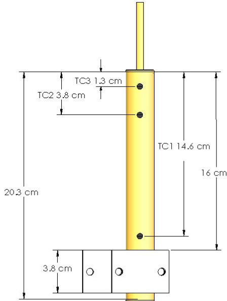
Figure 8. Location of thermocouples and heater block.
