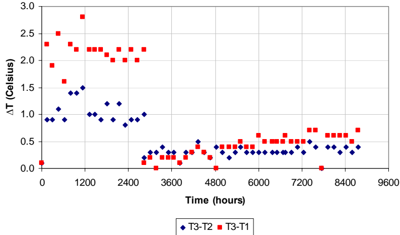
Figure 14. Low Temperature (Non-Condensable Gas) Measurements for Grade 7 Titanium Cylinder/CP-Titanium Screen/Water Heat Pipe 8, Operating at 550 K. Purged after 2837 hours of operation.
