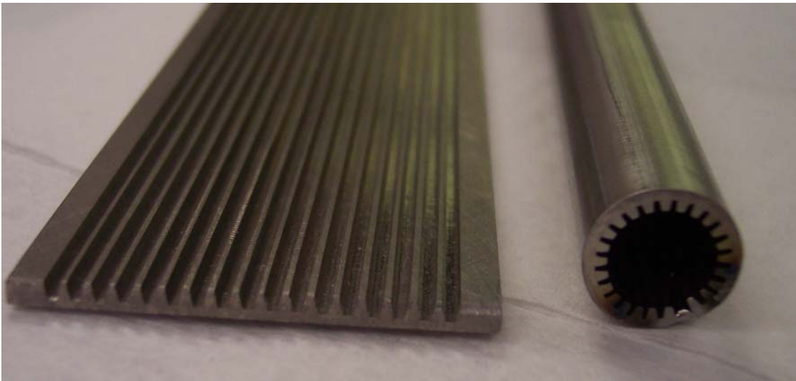
Figure 1. The solid groove heat pipes are fabricated from a flat plate.
