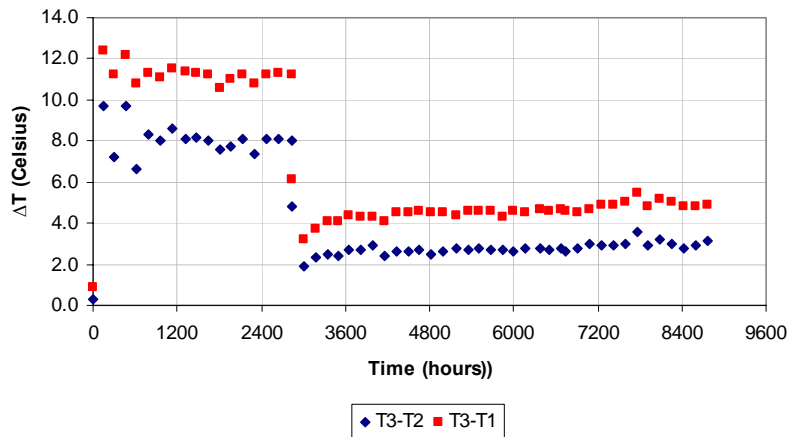
Figure 12. Low Temperature (Non-Condensable Gas) Measurements for CP Titanium Envelope/-35+60 Mesh CP-Titanium Sintered Powder/Water Heat Pipe 4, Operating at 550 K. Purged after 2837 hours of operation.
