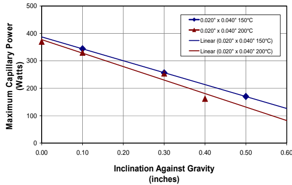
Figure 6. Typical Test Data and linear extrapolation (50 °C Delta T). 23 Grooves, 0.51 mm x 1.02 mm (0.020" x 0.040"), Titanium/Water Heat Pipe.
