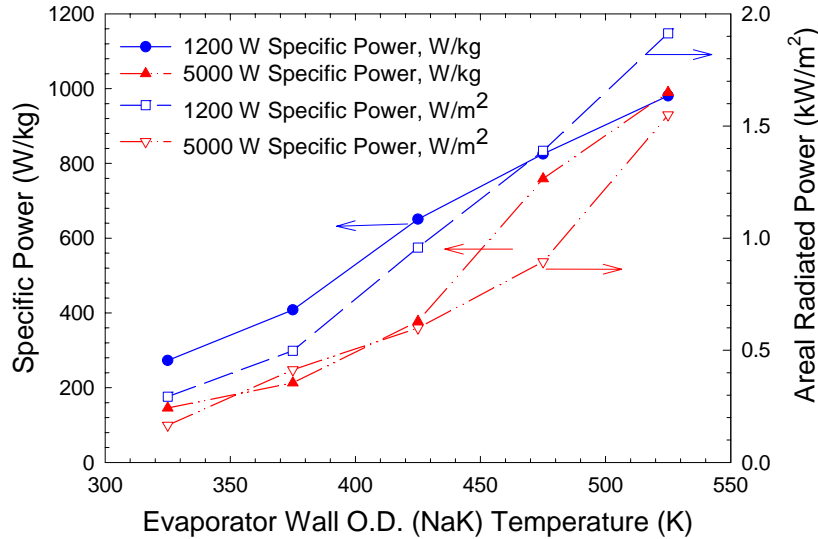
FIGURE 4. LHP Radiator Specific Power, Standard and Advanced Evaporators, 1000 W/m K Fins.
