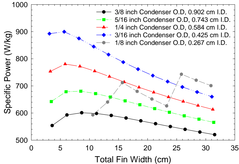
FIGURE 7. LHP Trade Study - Specific Power Versus Fin Width, 525 K, 600 W/m K Fin Thermal Conductivity.
