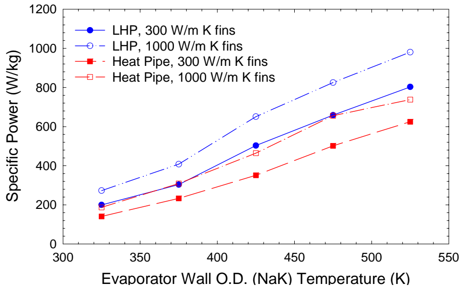
FIGURE 8. LHP Versus Heat Pipe Specific Power, 300 and 1000 W/m K Fins.
