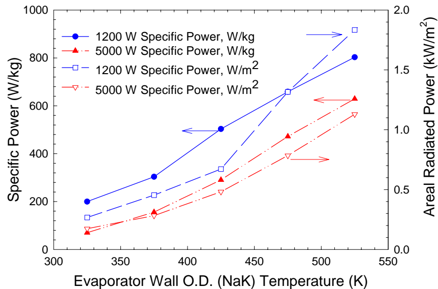
FIGURE 3. LHP Radiator Specific Power, Standard and Advanced Evaporators, 300 W/m K Fins.
