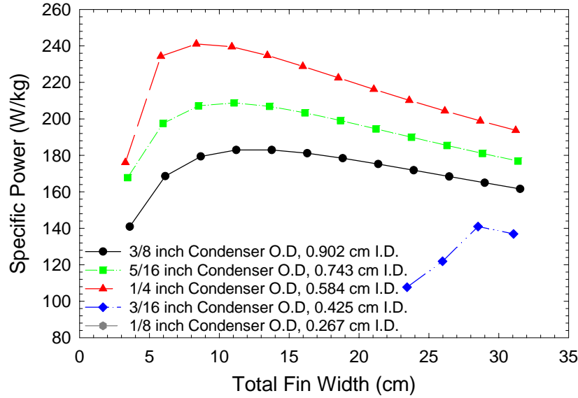
FIGURE 6. LHP Trade Study - Specific Power Versus Fin Width, 325 K, 600 W/m K Fin Thermal Conductivity.
