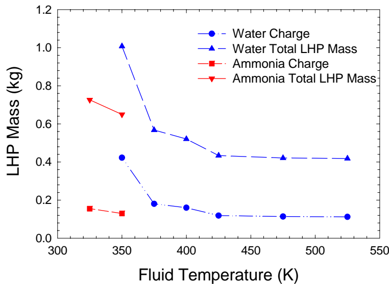
FIGURE 2. LHP Standard Evaporator, Fluid and Total LHP Mass for the Standard Evaporator with 1200 W Power.
