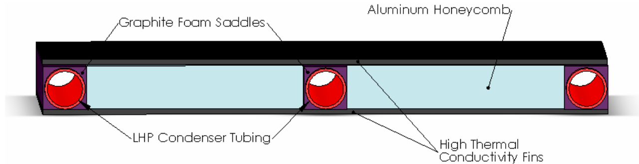
FIGURE 1. Cutaway Section Through The Panel.
