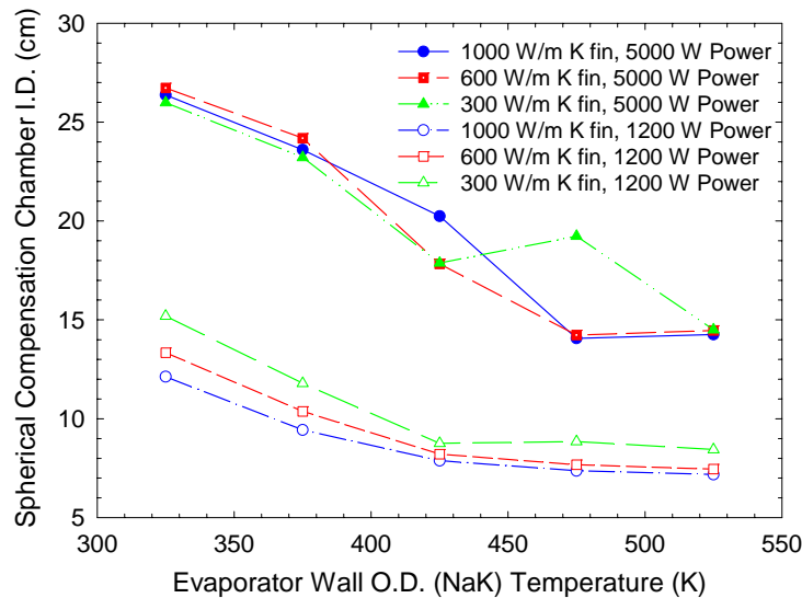
FIGURE 5. LHP Spherical Compensation Chamber Diameter. Standard and Advanced Powers, 300, 600, and 1000 W/m K Fins. The Advanced Power Designs Have A Much Larger Compensation Chamber, Due to the Longer Line Lengths.
