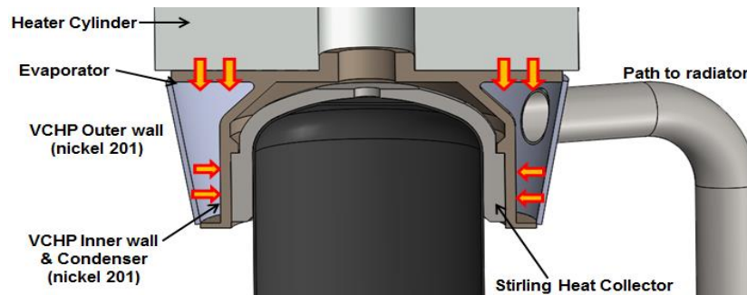
FIGURE 3. Cross section of the Stirling hot end, VCHP annulus and heater cylinder after assembly.
