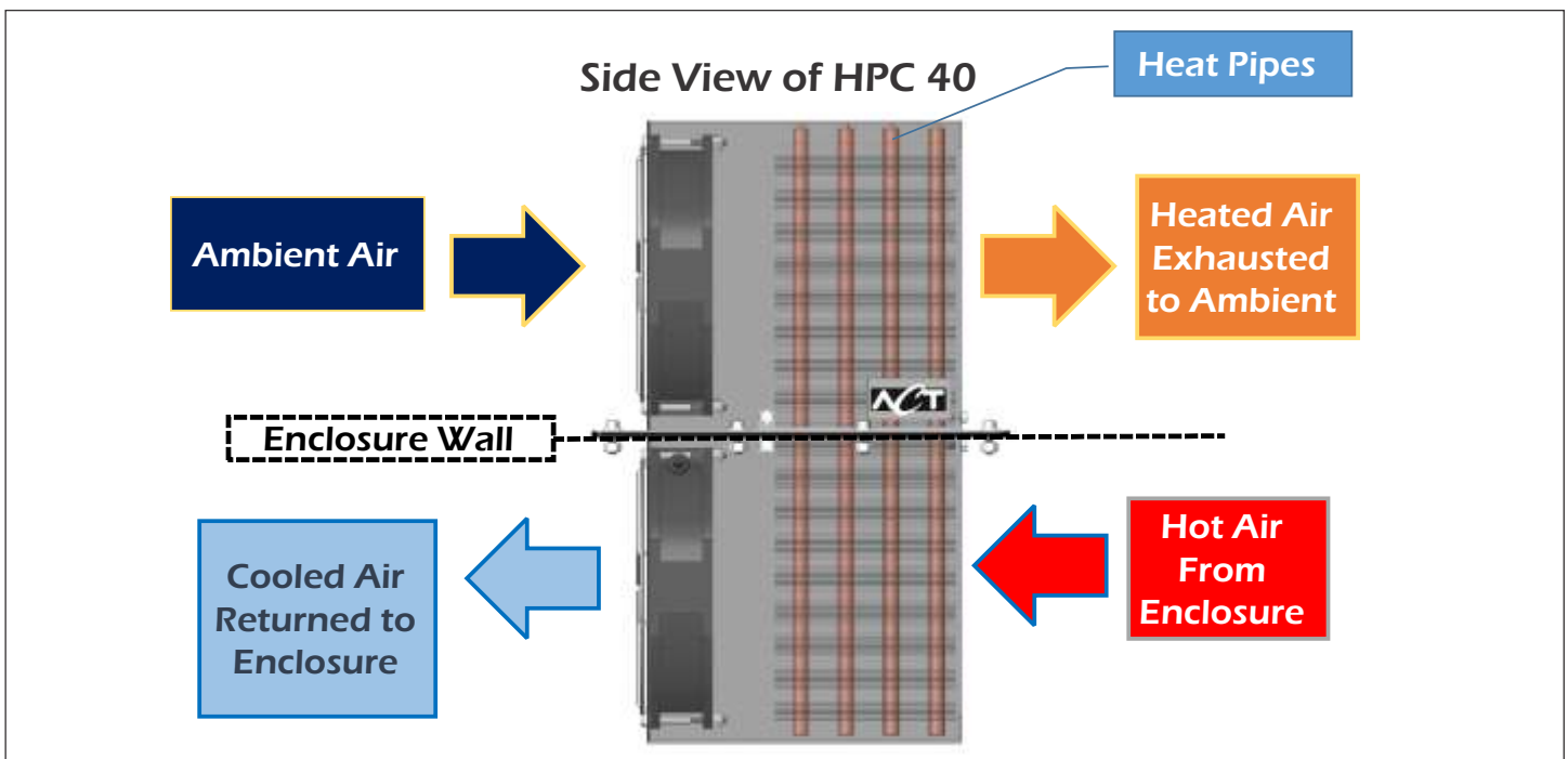
Figure 1 : Side View of ACT-HPC-40 with arrows showing the airflow patterns of the internal and external air streams
