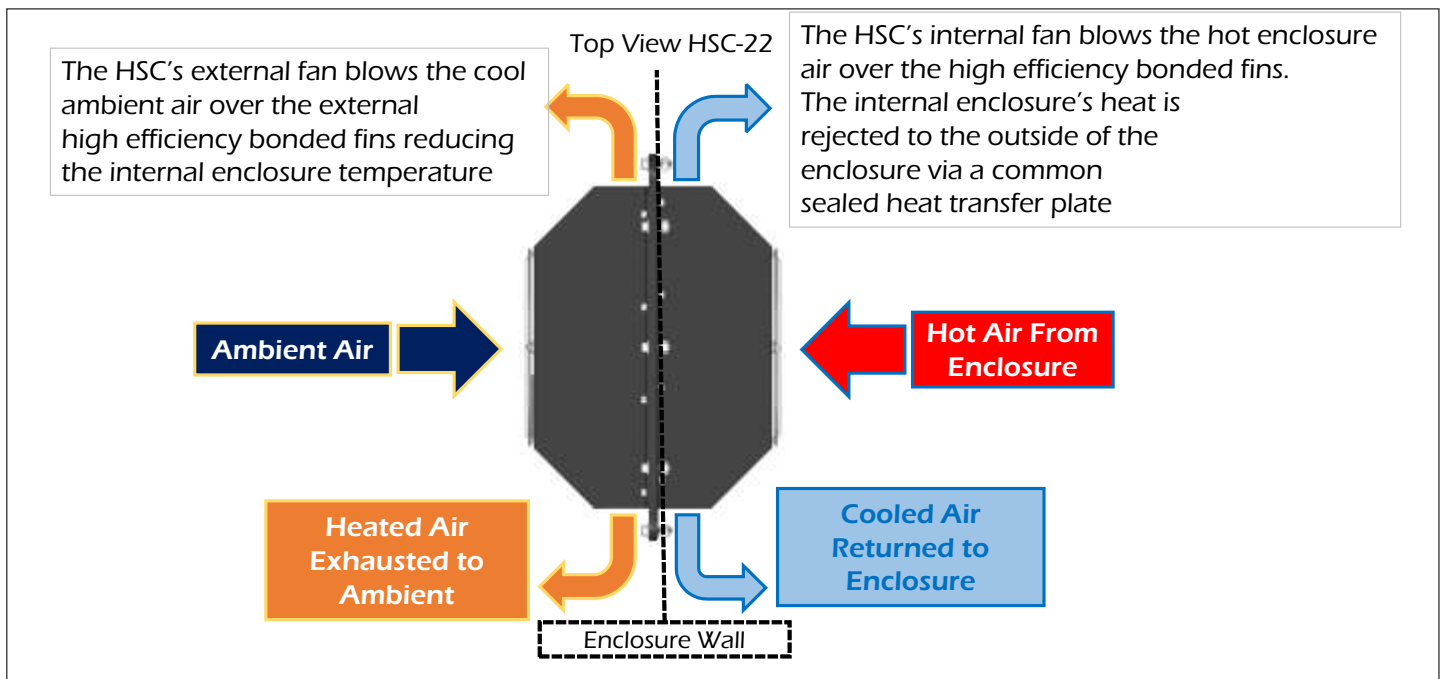
Figure 1 : Top View of ACT-HSC-22 with arrows showing the airflow patterns of the internal and external air streams
