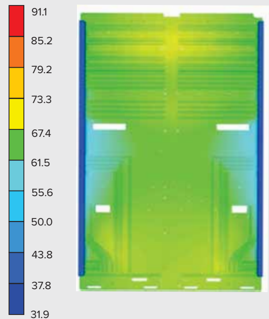
(b) Temperature Profile of a HiK™ Plate that has the same components as Figure A above.
