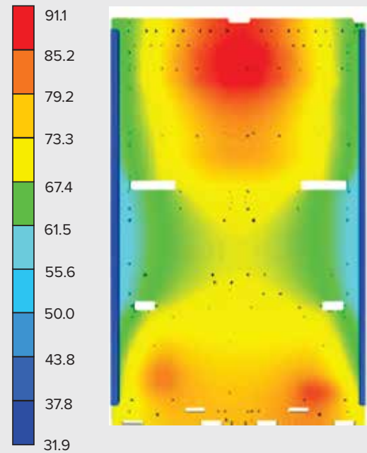
(a) Temperature Profile of an edge cooled aluminum plate with various high powered electronic components
