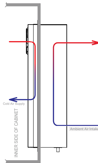
AIR FLOW DIAGRAM
