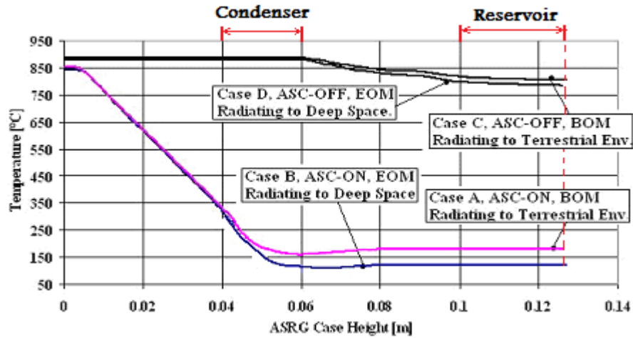
FIGURE 5. Temperature distributions along the entire VCHP for all four cases.
