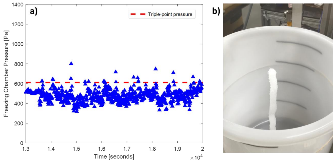
Figure 4. a) The steady state pressure in the freezing chamber when the boiler temperature is 80°C. The pressure fluctuates around 470 Pa, which is below the triple-point pressure of water. b) As the water drips out of the needle inside the freezing chamber, the evaporation at a pressure below the triple point results in the formation of ice inside the freezing chamber.
