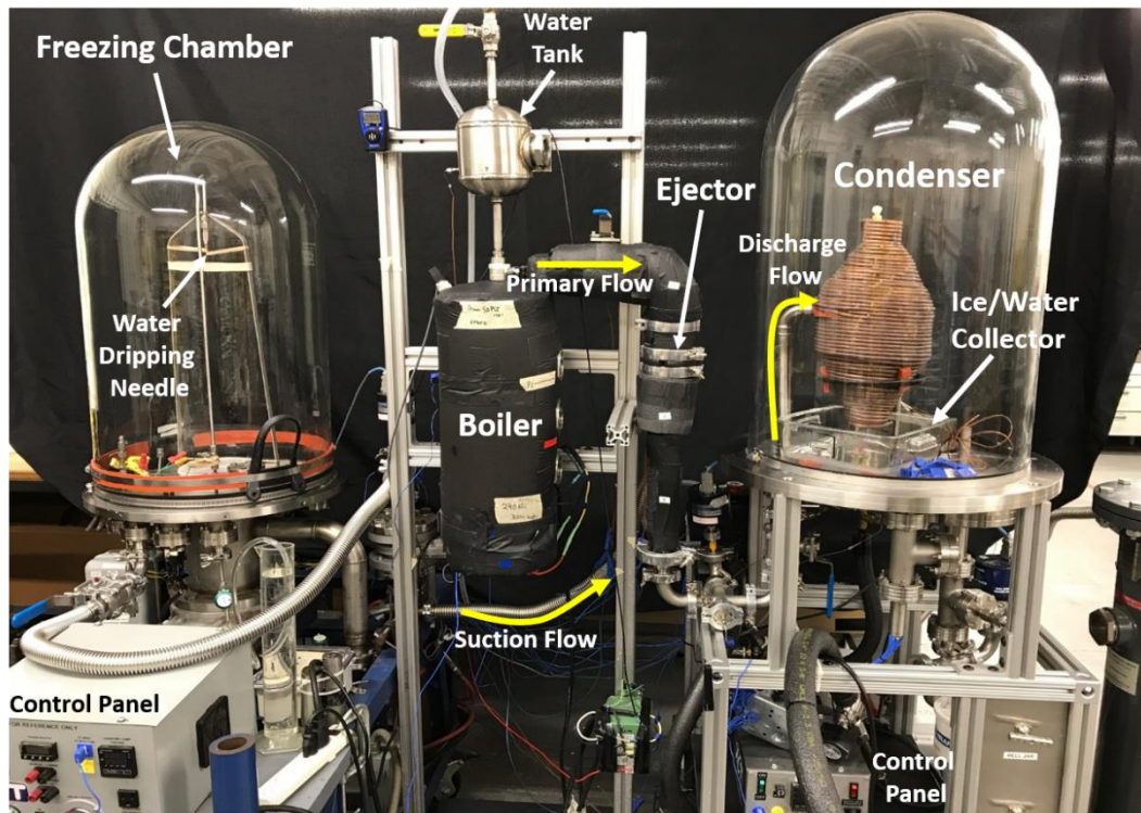
Figure 3. Experimental setup for the complete system of vacuum freezing triple-point desalination.
