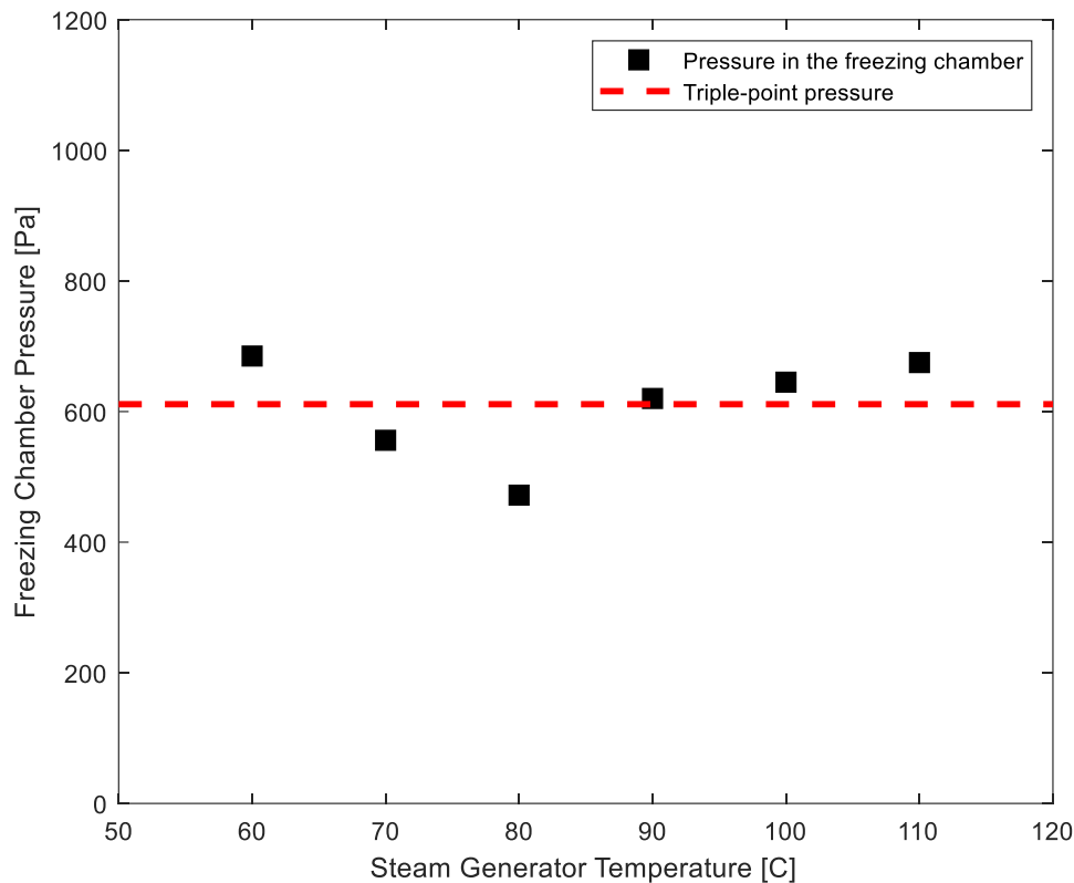
Figure 5. The steady state pressure in the freezing chamber as a function steam generator temperature (i.e., ejector primary flow temperature). For boiler temperatures at 70°C, 80°C and 90°C, we observed ice formation inside the freezing chamber during the water dripping process since the pressure in the freezing chamber can be maintained near or below the triple point pressure.
