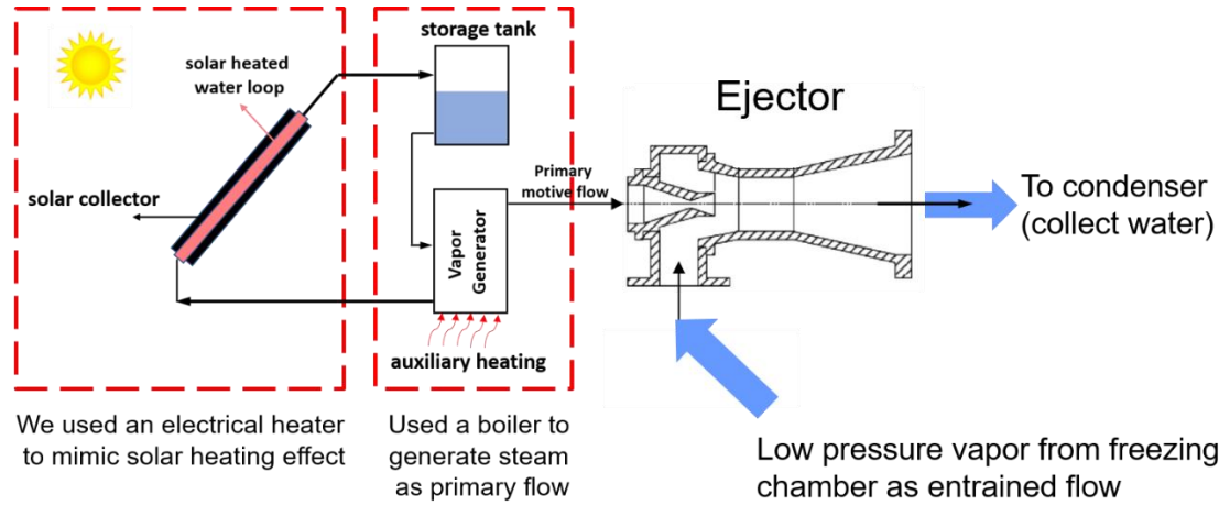
Figure 1. Schematic of the experimental setup for the ejector system that connects steam generator/boiler (provides primary flow), freezing chamber (provides suction/entrained flow) and condenser (collects water from primary and entrained flows).
