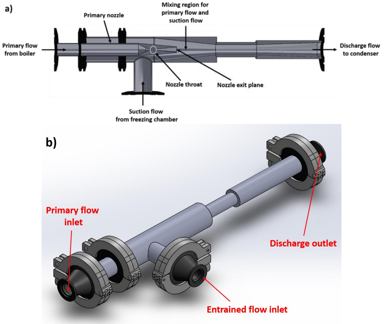
Figure 2. a) Cross-sectional view of the ejector internal structure. b) Solidworks design of the ejector.
